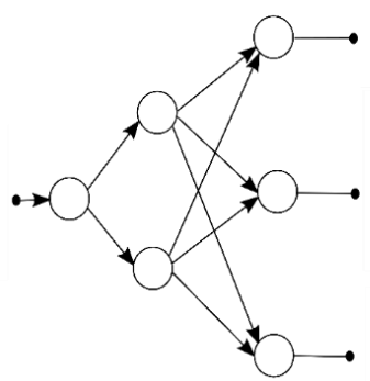
DECODER
