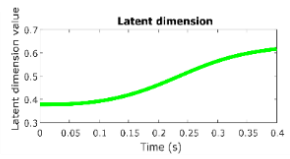
LATENT SPACE
