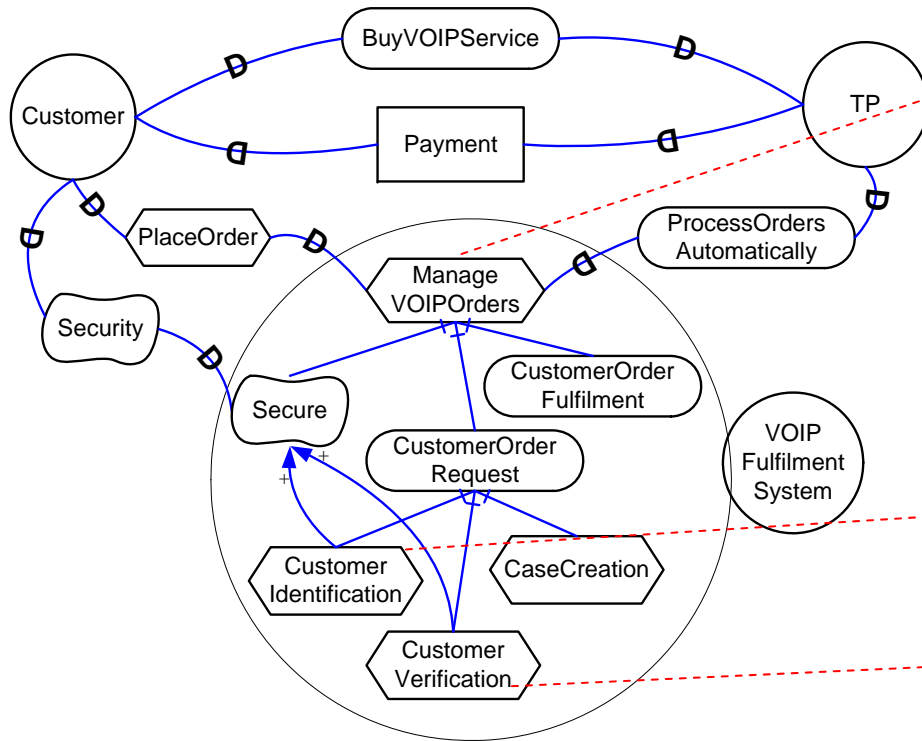
Early requirements (i*)
