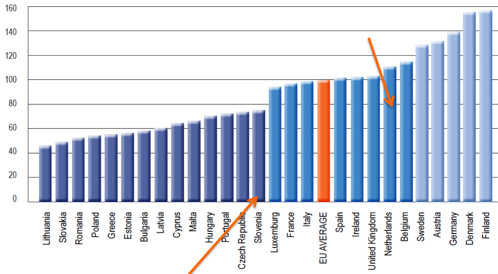
EU-27 Eco-Innovation Scoreboard: composite index
