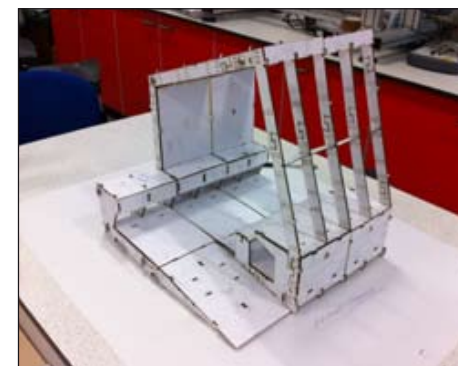
Scale model of the Chelmsford WikiHouse
