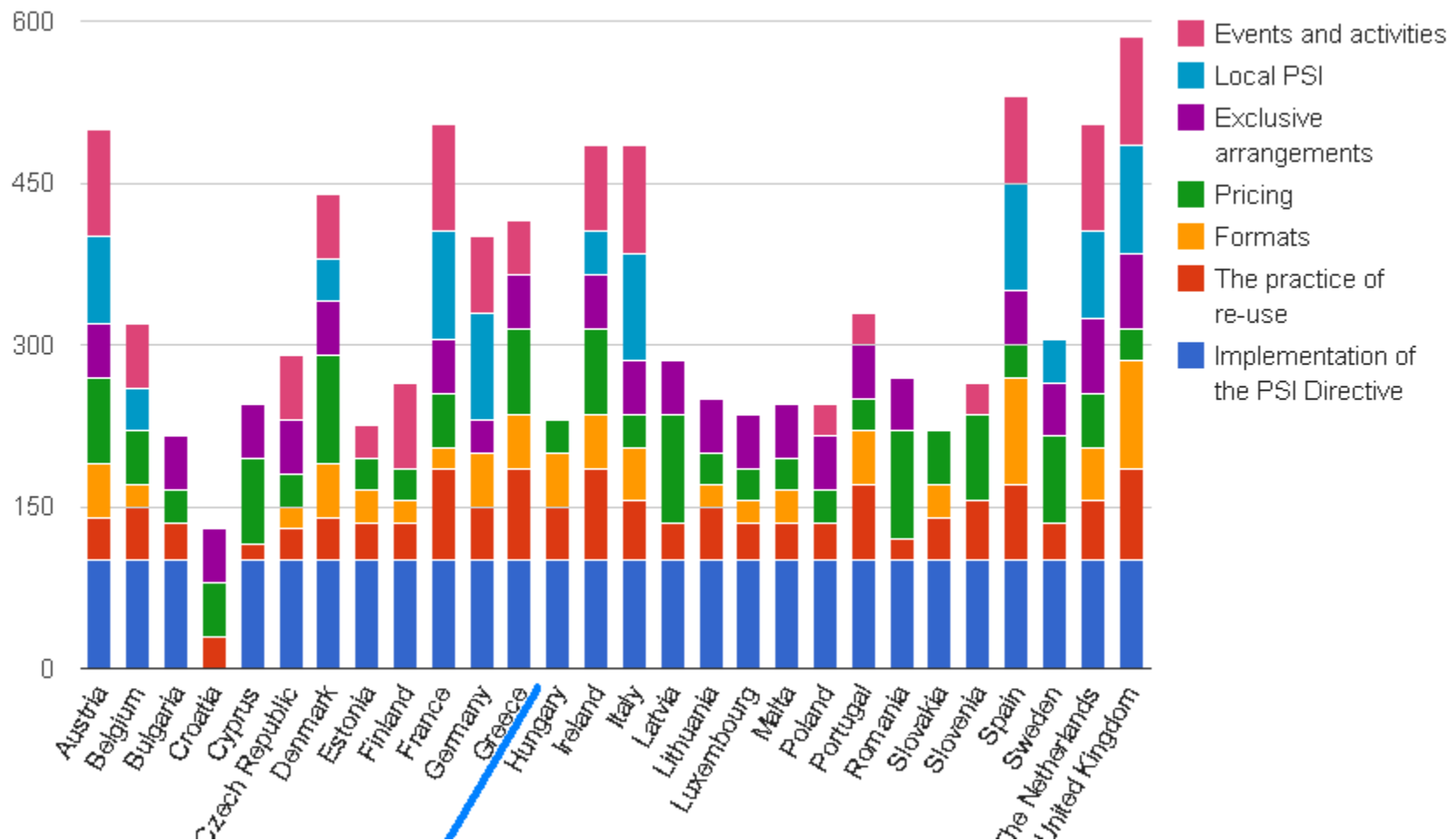
Aggregated Scores
