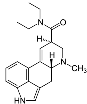
LSD
