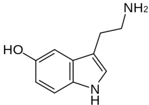
Serotonin
